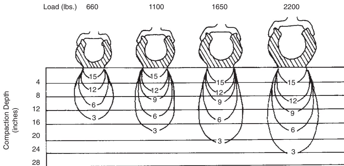
Figure 3. The effect of various tractor loads on soil compaction.
